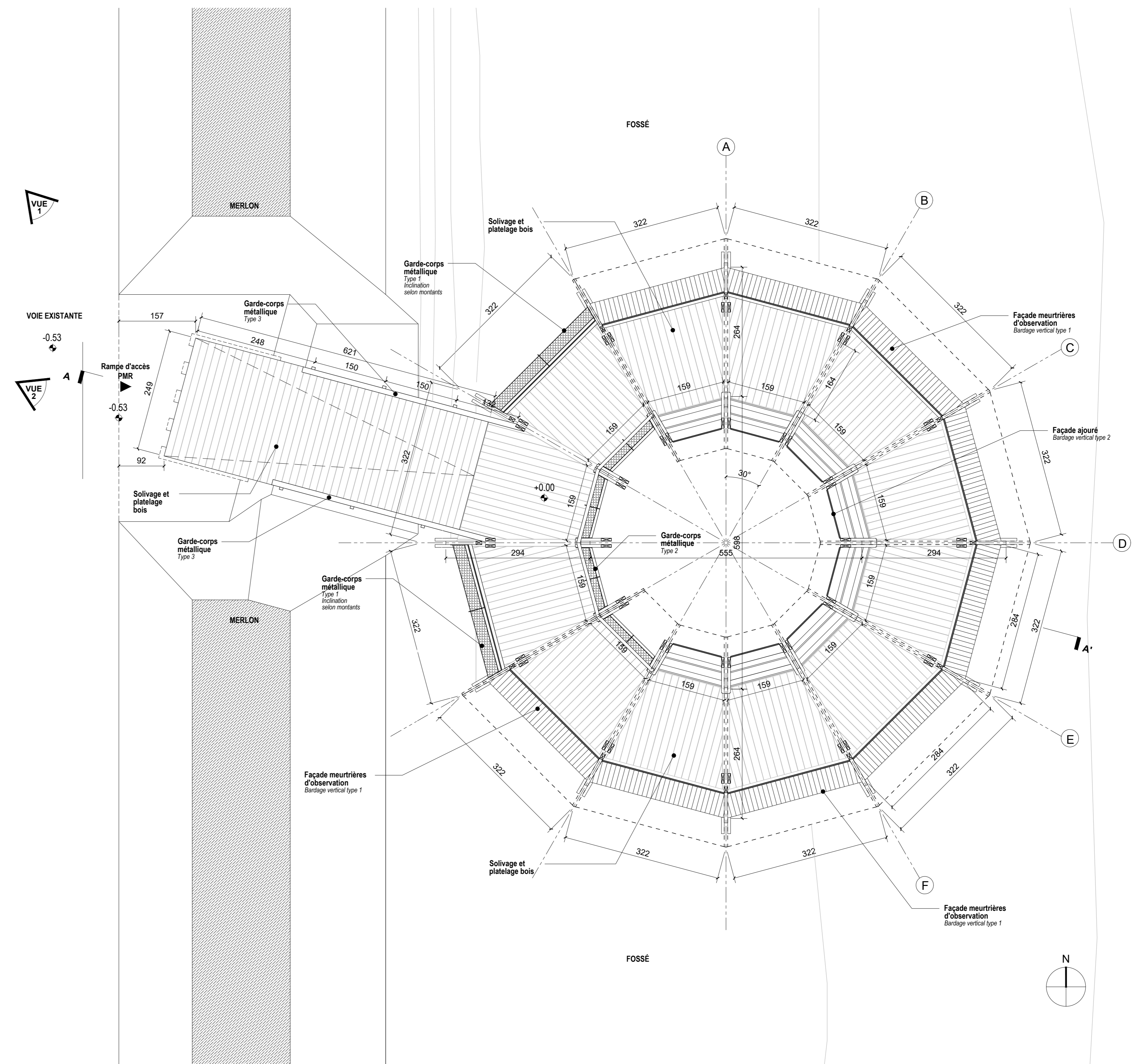
PLAN GENERAL ECH 1:50
